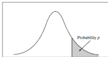
Students t-distribution Table of Values
